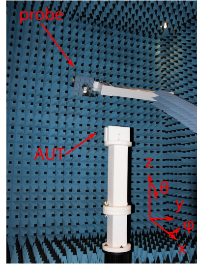
Fig. 3: Antenna under test (AUT) and coordinate system inside the near-field anechoic chamber.
