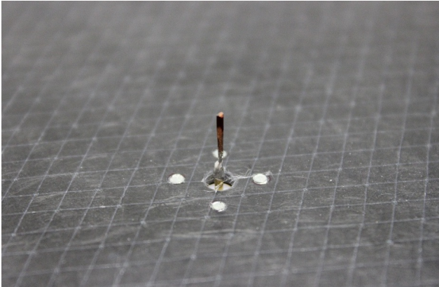
Fig. 2: Wire monopole antenna for 5.9 GHz on the CFC ground plane.
