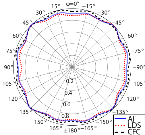
(a) Radiation pattern of wire monopoles
