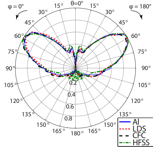
(b) Radiation pattern of LDS monopoles
