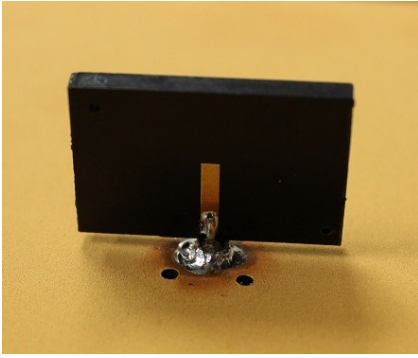
Fig. 1: Monopole antenna in MID technology. The outer conductor of a semi-rigid coaxial cable is soldered to the conductive LDS-layer of the ground plane. The inner conductor of the coaxial cable is soldered to the LDS monopole on the plastic carrier. The four holes designed for an SMA-flange remain unused.
