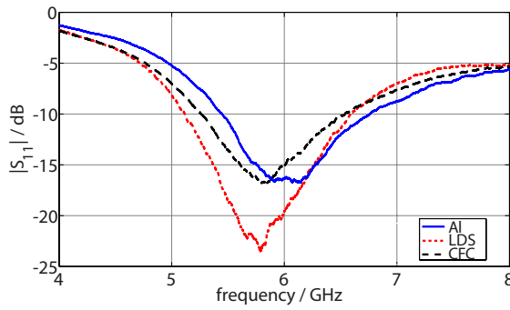
(a) Return loss of wire monopoles
