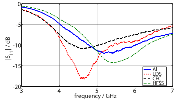
(b) Return loss of LDS monopoles
